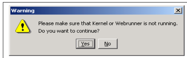
Figure 6.3: Warning Message
