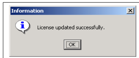
Figure 6.4: Confirmation Message
