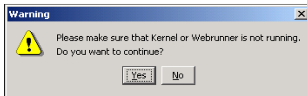
Figure 3: Warning Message
