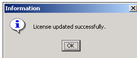
Figure 4: Confirmation Message
